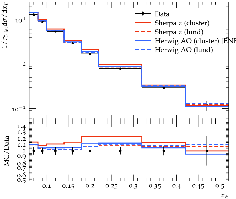
Scaled energy fraction for \pi^0 in 1st jet (3-jet events)
