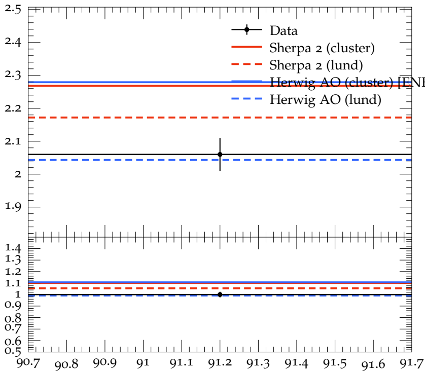
Mean K_S + K_L multiplicity
