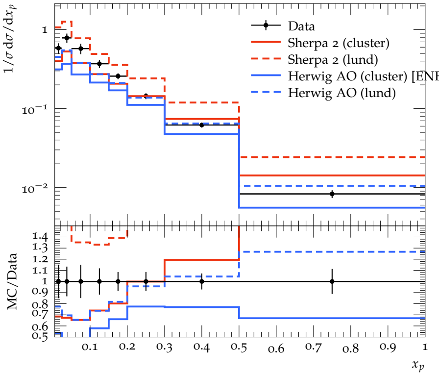
\phi spectrum
