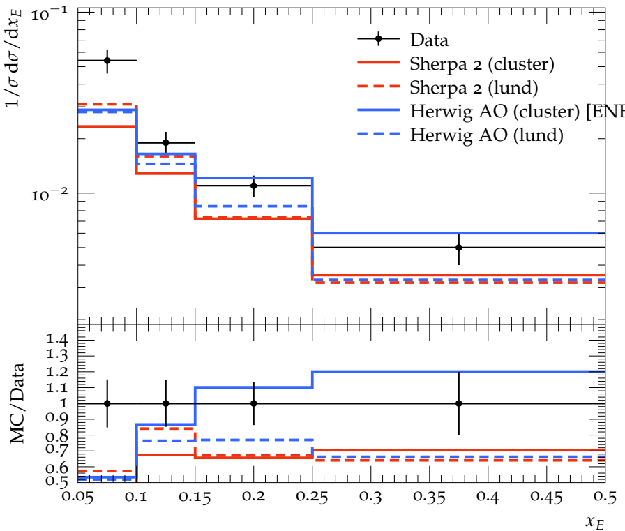
\Xi^0(1530) spectrum
