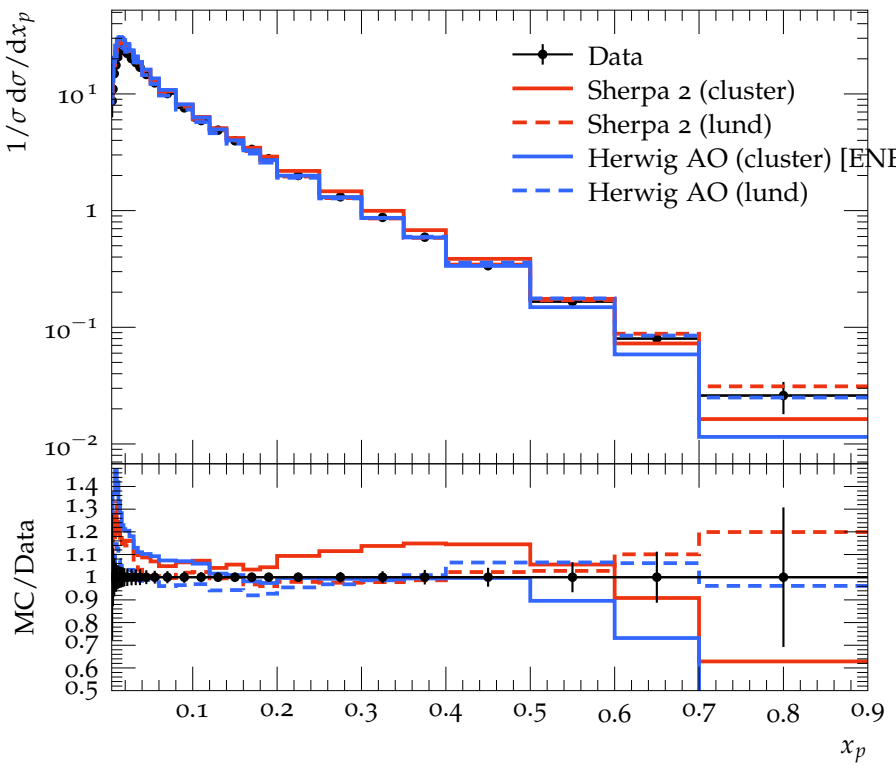
K^0 spectrum
