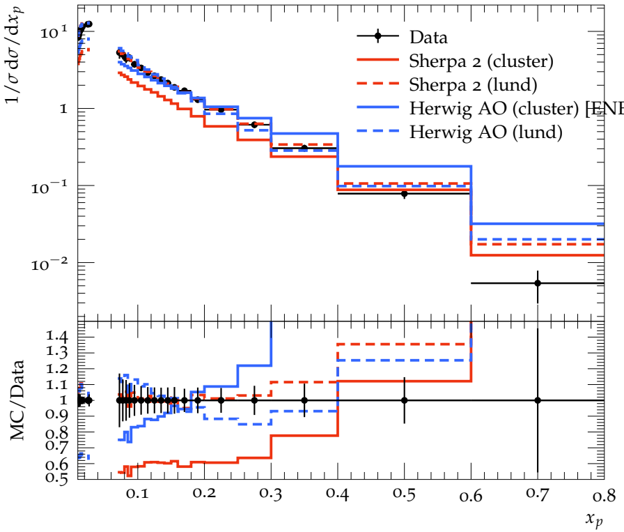
p spectrum
