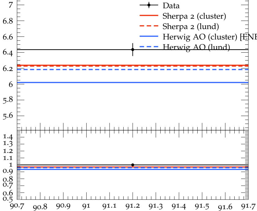
Mean charged multiplicity for rapidity |Y| < 1.0
