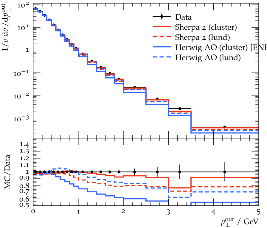
Out-of-plane p_T in GeV w.r.t. sphericity axes (charged)
