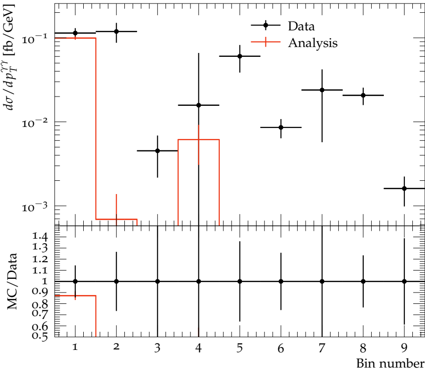
1D differential xsection vs p_T^{\gamma\gamma} in bins of p_T^{\gamma\gamma j}
