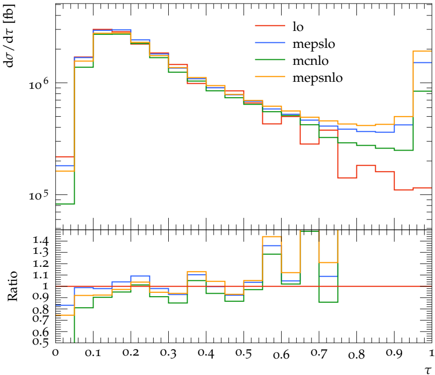
1-jettiness \tau in given bins of x and Q^2
