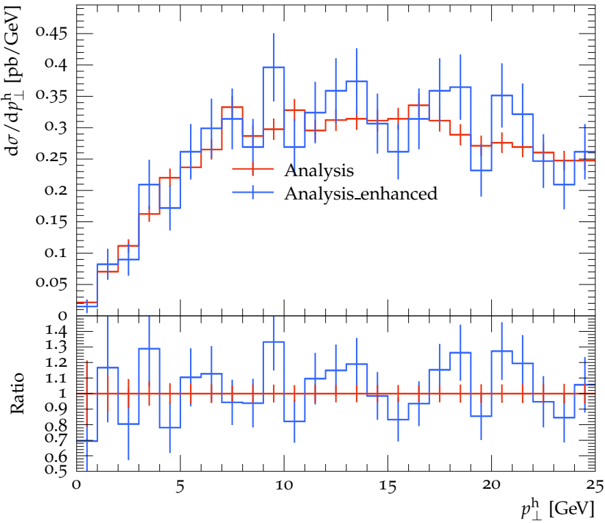
Higgs boson p_{\perp} in peak region
