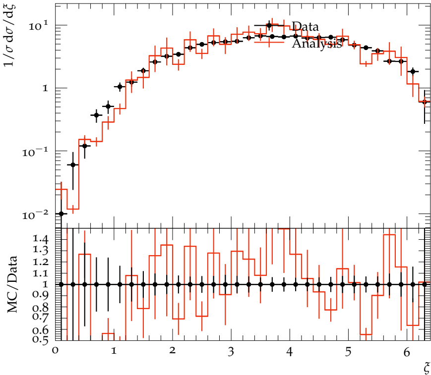
Log of the scaled momentum at 161 GeV
