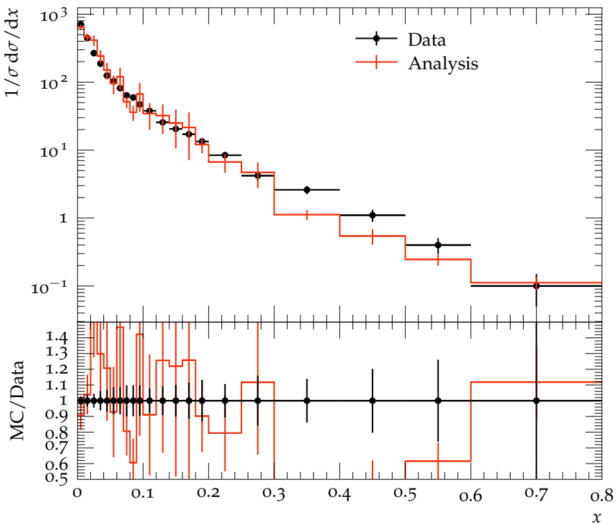
Scaled momentum at 161 GeV
