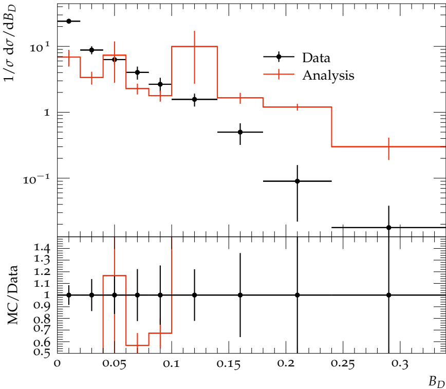
Difference of the jet broadenings ( E_{\text{CMS}} = 161 \text{ GeV} )
