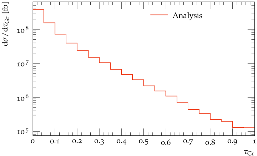
Groomed 1-jettiness \tau_{\text{Gr}} with z_{\text{cut}} = 2
