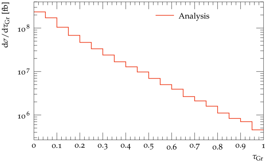
Groomed 1-jettiness \tau_{\text{Gr}} with z_{\text{cut}} = 1
