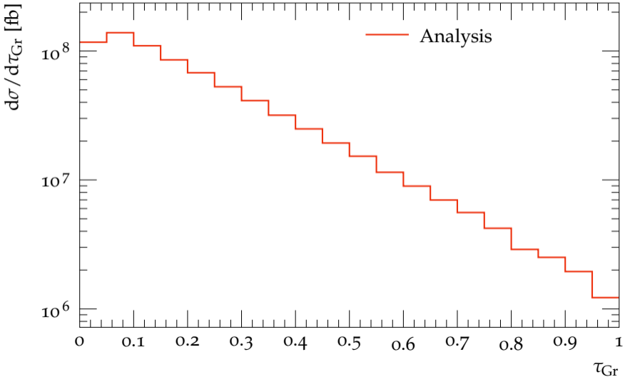
Groomed 1-jettiness \tau_{\text{Gr}} with z_{\text{cut}} = 0.5
