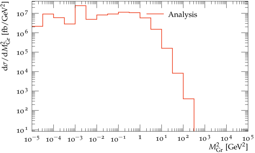
Groomed invariant mass M_{\text{Gr}}^2 with z_{\text{cut}} = 1
