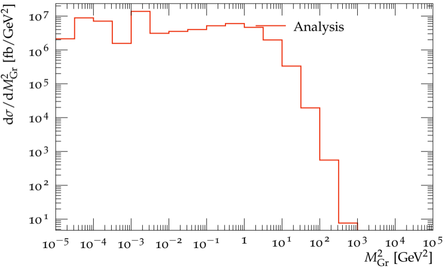
Groomed invariant mass M_{\text{Gr}}^2 with z_{\text{cut}} = 0.5
