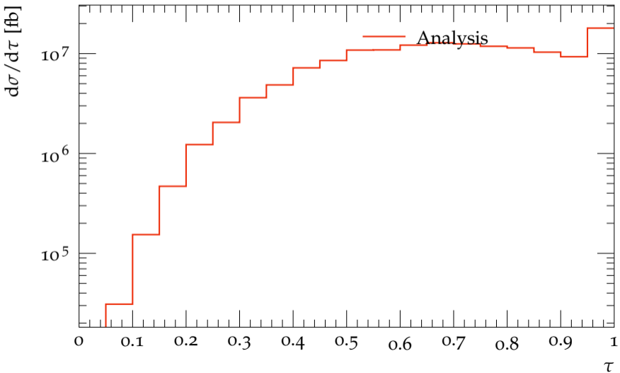
1-jettiness \tau in given bins of x and Q^2
