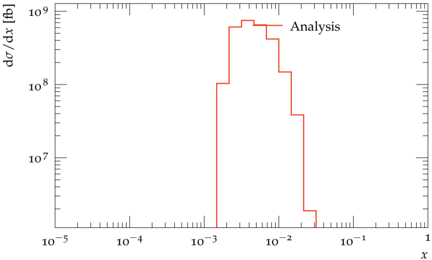
Distribution of Bjorken- x in bin of Q^2
