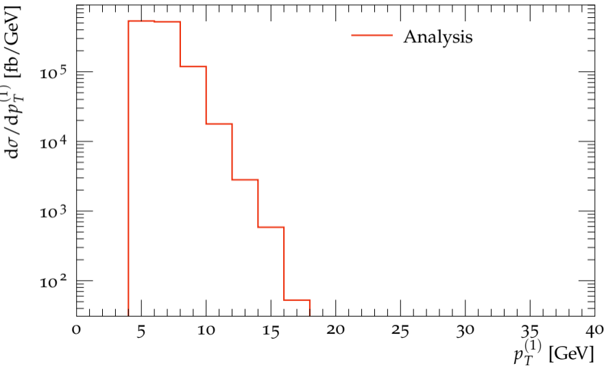
Distribution of leading jet transverse momentum in bin of Q^2
