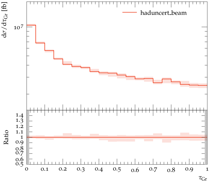
Groomed 1-jettiness \tau_{\text{Gr}} with z_{\text{cut}} = 2
