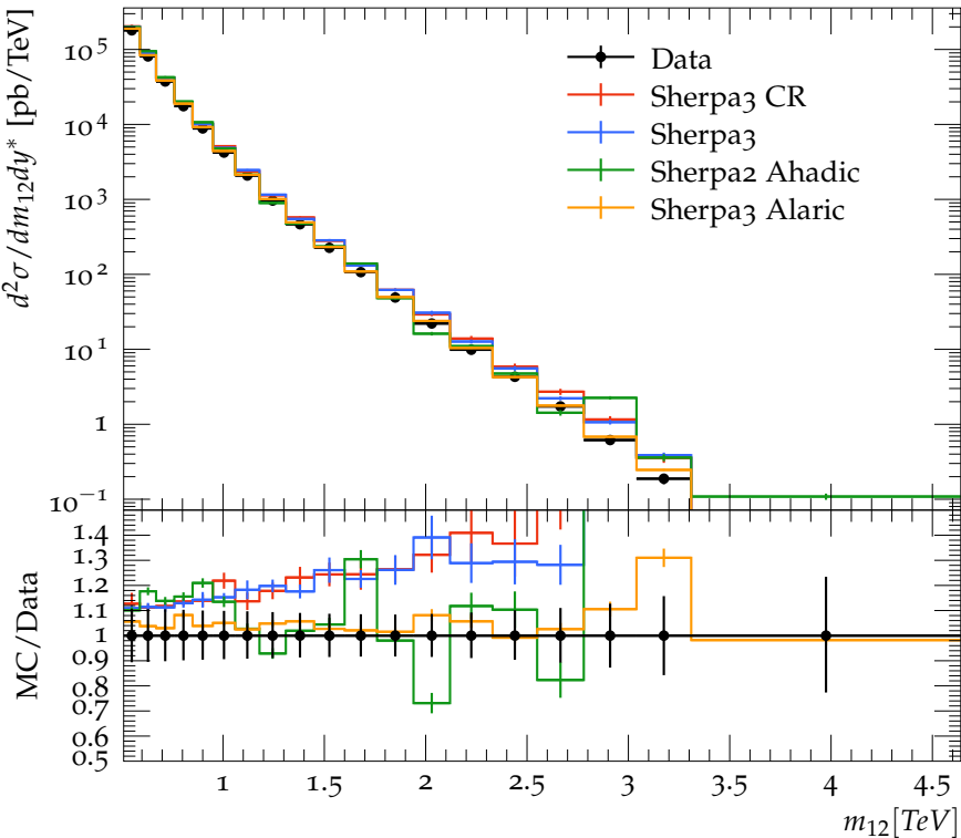
Dijet double-differential cross sections ( 1.0 < y^* < 1.5 ), R=0.6
