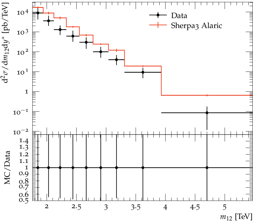
Dijet double-diff. x-section, anti- k_t 0.4 ( 3.5 \leq y^* < 4.0 )
