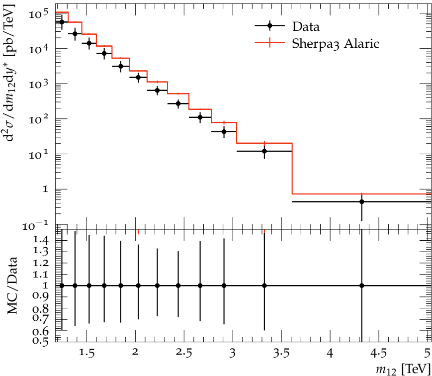
Dijet double-diff. x-section, anti- k_t 0.4 ( 3.0 \leq y^* < 3.5 )
