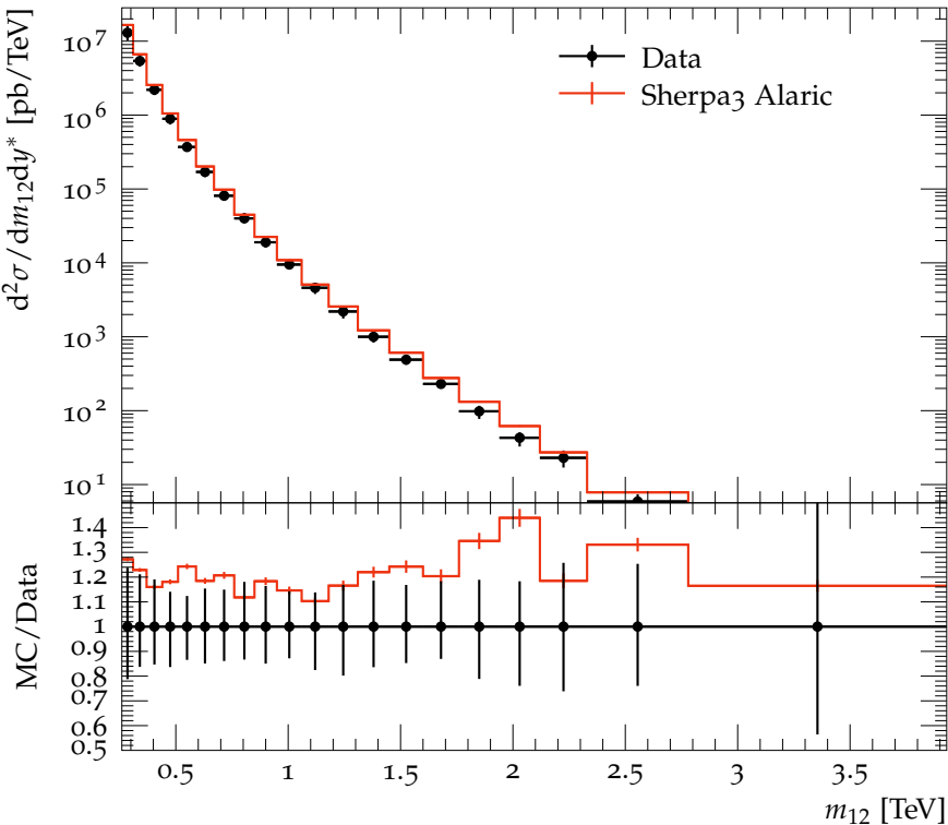
Dijet double-diff. x-section, anti- k_t 0.4 ( 1.5 \leq y^* < 2.0 )
