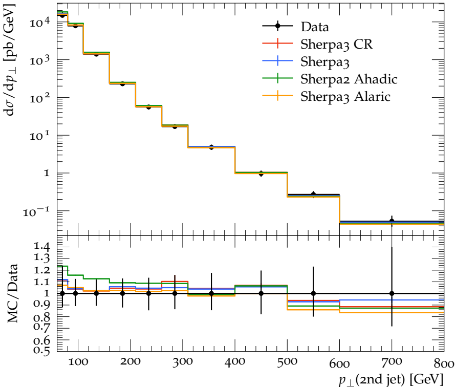
Transverse momentum of the 2nd leading jet ( R = 0.4 )
