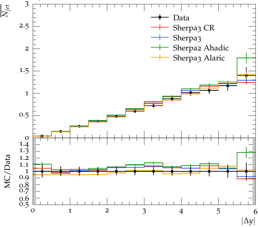
\overline{N}_{jet} vs |\Delta y| for 90 < \overline{P}_T < 120 , Leading Jet
