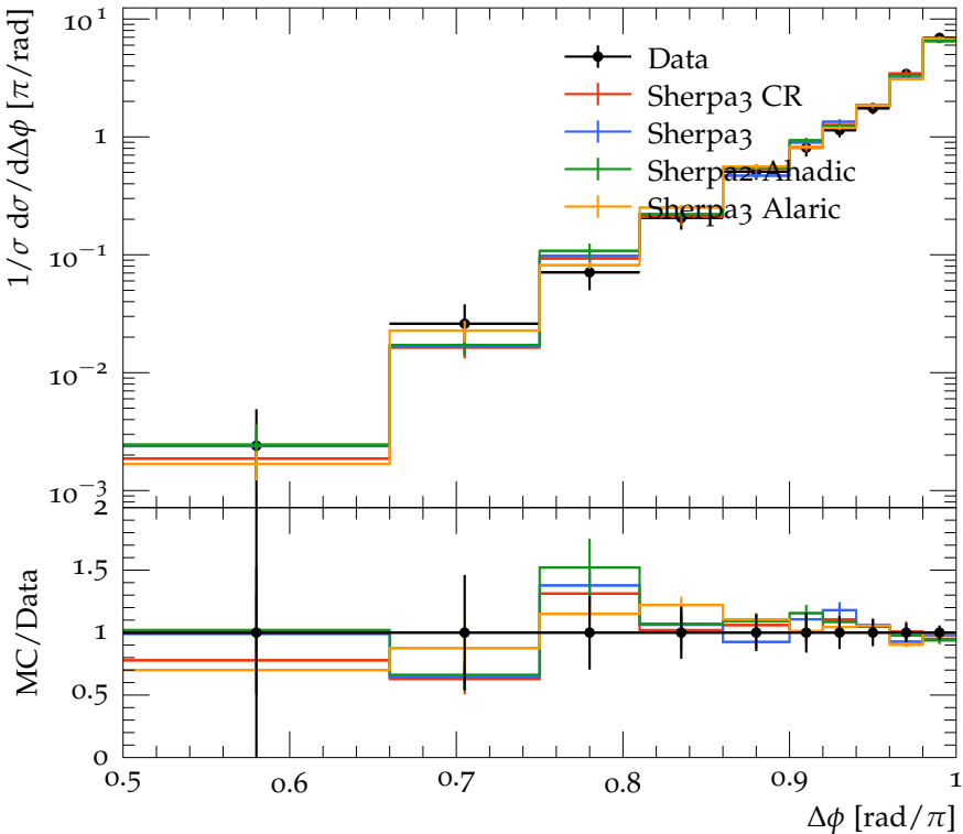
Dijet azimuthal decorrelations for 500 < p_{\perp}^{\max}/\text{GeV} < 600
