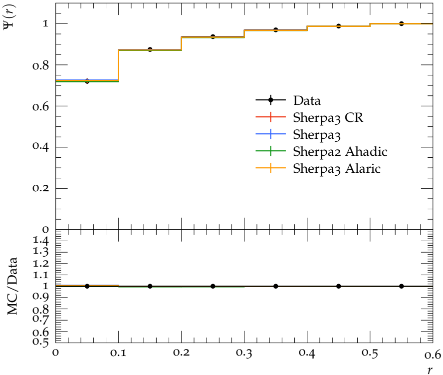
Jet shape \Psi for p_{\perp} \in 260\text{--}310 GeV, y \in 0.3\text{--}0.8
