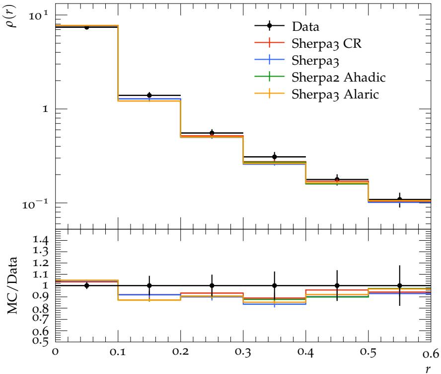
Jet shape \rho for p_{\perp} \in 210\text{--}260 GeV, y \in 2.1\text{--}2.8
