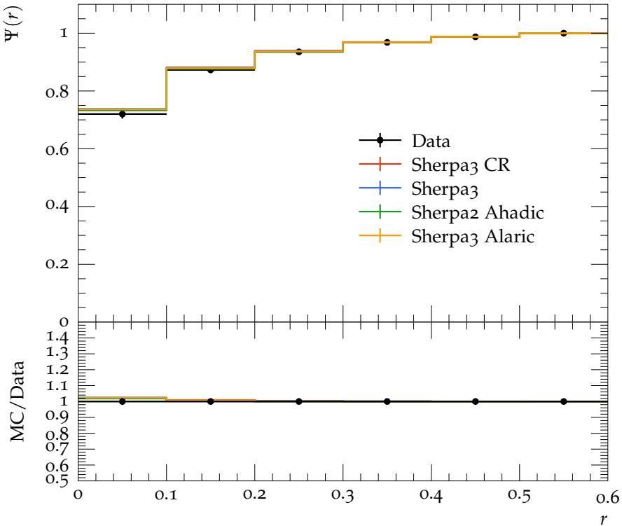
Jet shape \Psi for p_{\perp} \in 210\text{--}260 GeV, y \in 1.2\text{--}2.1
