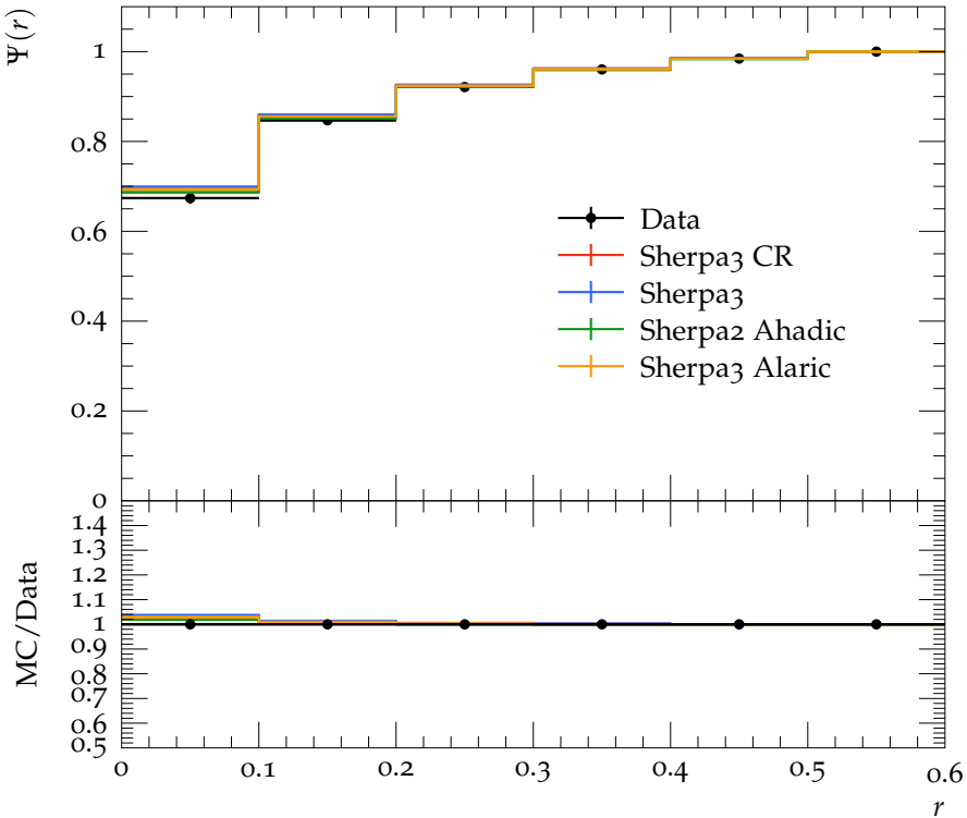
Jet shape \Psi for p_{\perp} \in 160\text{--}210\text{ GeV} , y \in 0.0\text{--}2.8
