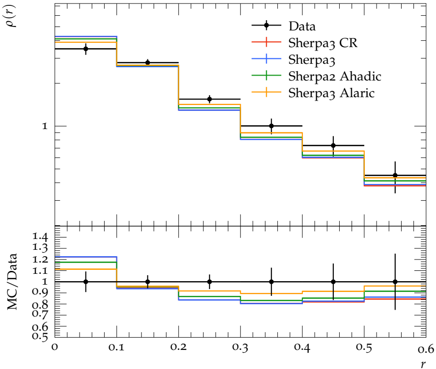
Jet shape \rho for p_{\perp} \in 30\text{--}40\text{ GeV} , y \in 1.2\text{--}2.1
