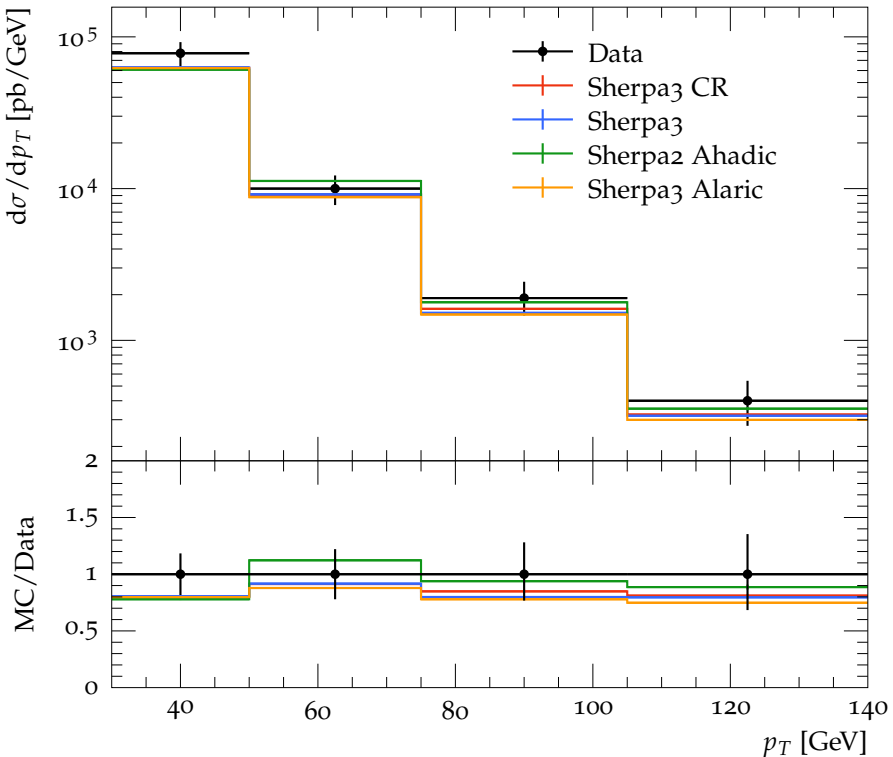
Muon tagged b -jet p_T for |y| < 2.1 , anti- k_T , R = 0.4
