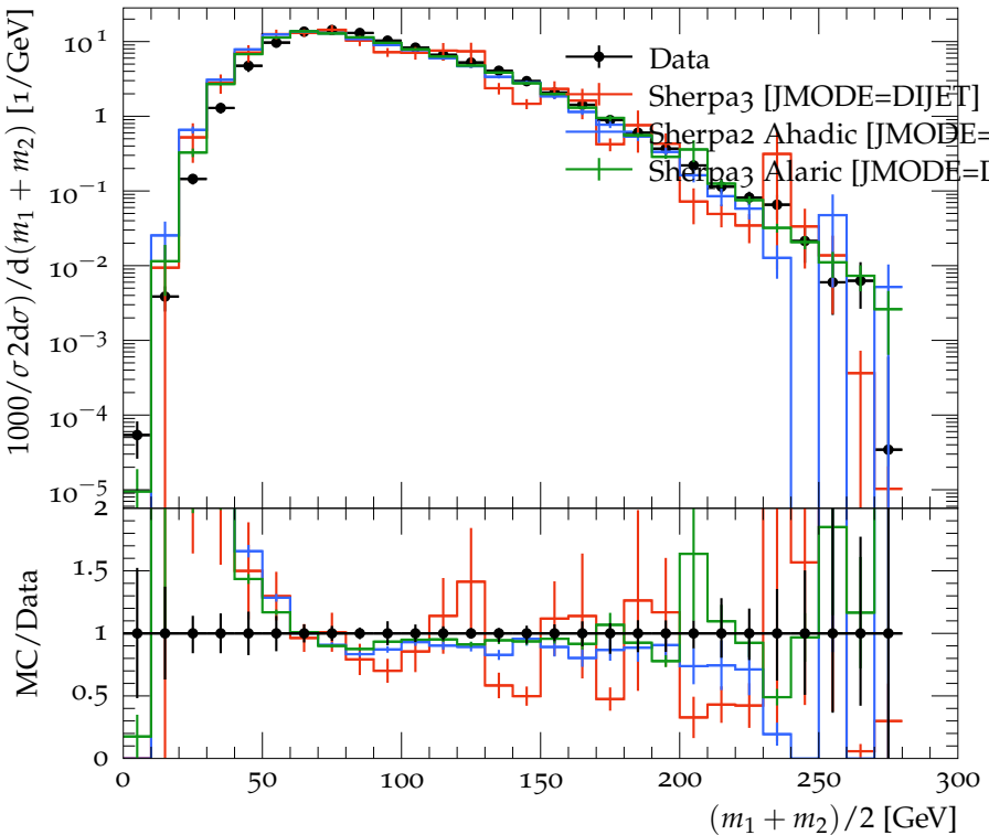
Ungroomed AK 7 dijets, (p_T^1 + p_T^2)/2 = 600\text{--}800 GeV
