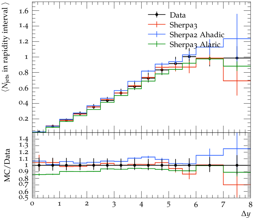
\langle N_{\text{jets}} \text{ in rapidity interval} \rangle as a function of \Delta\gamma
