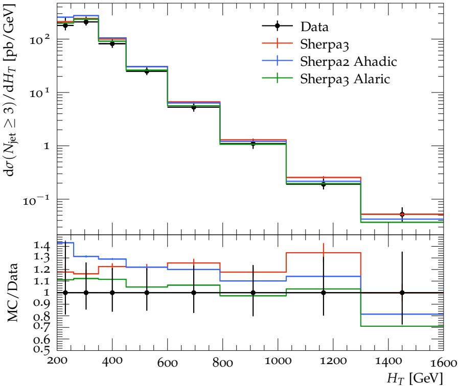
H_T for events with N_{\text{jet}} \geq 3 ( R = 0.4 )
