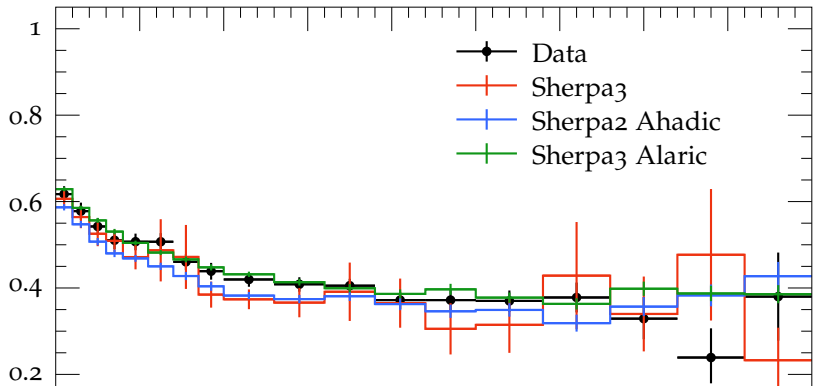
Gap fraction vs \overline{P_T} for 2.0 < |\Delta y| < 3.0 , Fwd/Bwd
