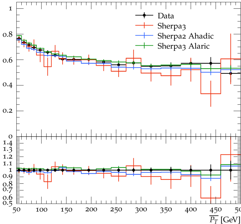
Gap fraction vs \overline{P_T} for 1.0 < |\Delta y| < 2.0 , Fwd/Bwd
