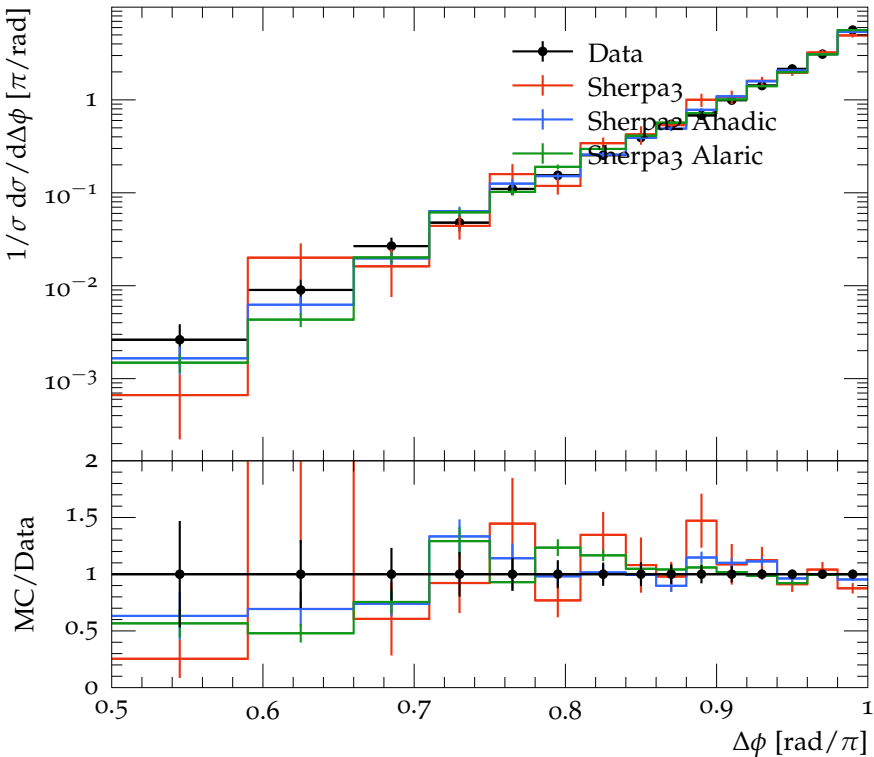
Dijet azimuthal decorrelations for 310 < p_{\perp}^{\max}/\text{GeV} < 400
