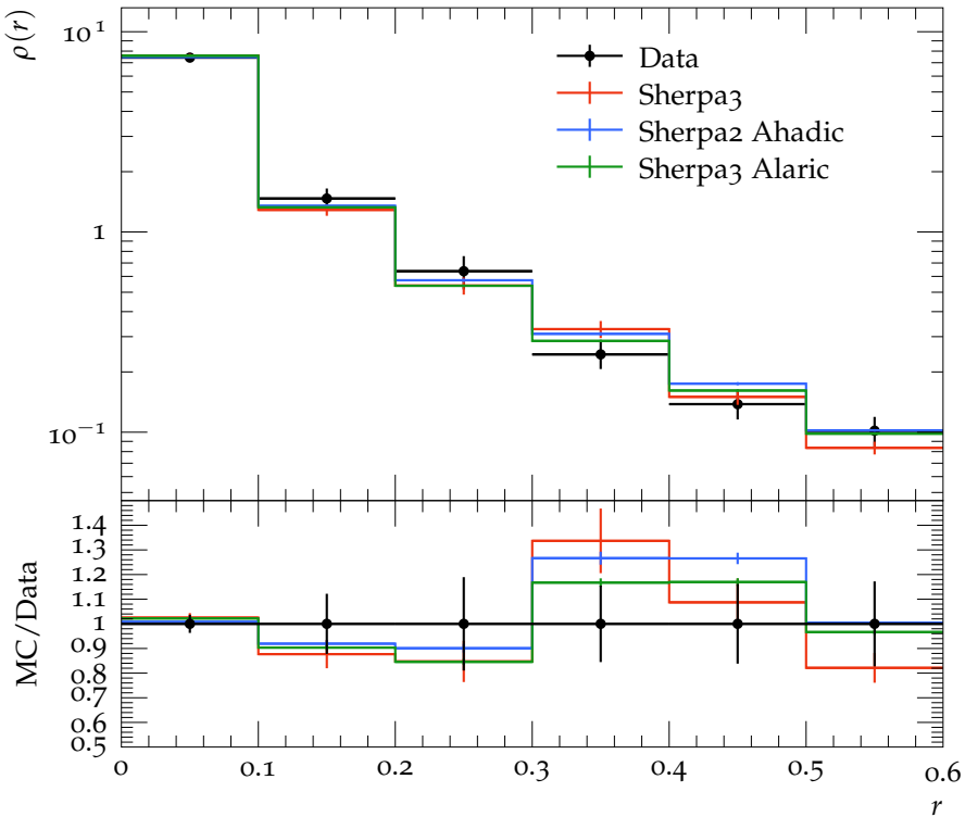
Jet shape \rho for p_{\perp} \in 400\text{--}500 GeV, y \in 0.0\text{--}0.3
