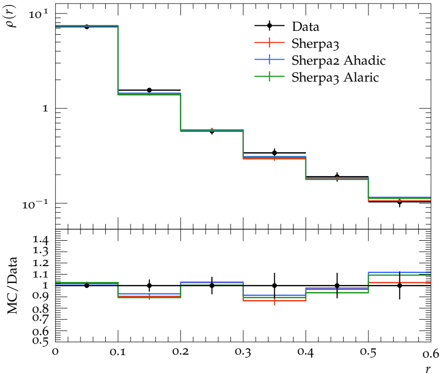
Jet shape \rho for p_{\perp} \in 310\text{--}400 GeV, y \in 0.3\text{--}0.8
