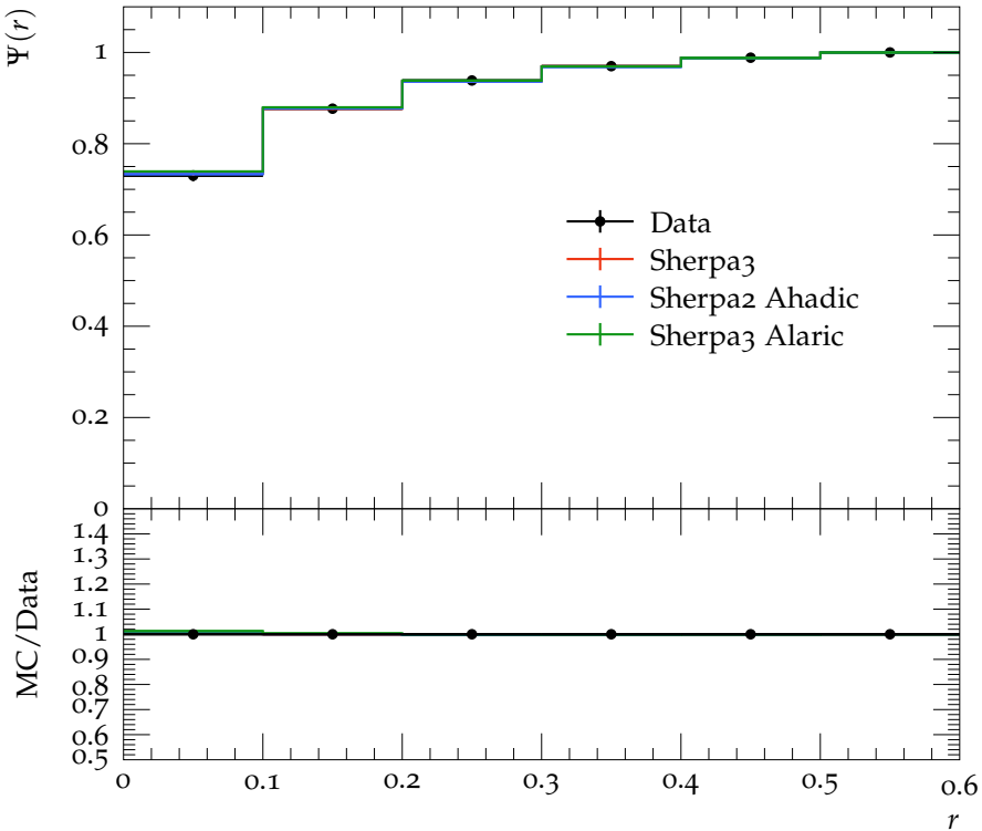
Jet shape \Psi for p_{\perp} \in 260\text{--}310\text{ GeV} , y \in 0.0\text{--}2.8
