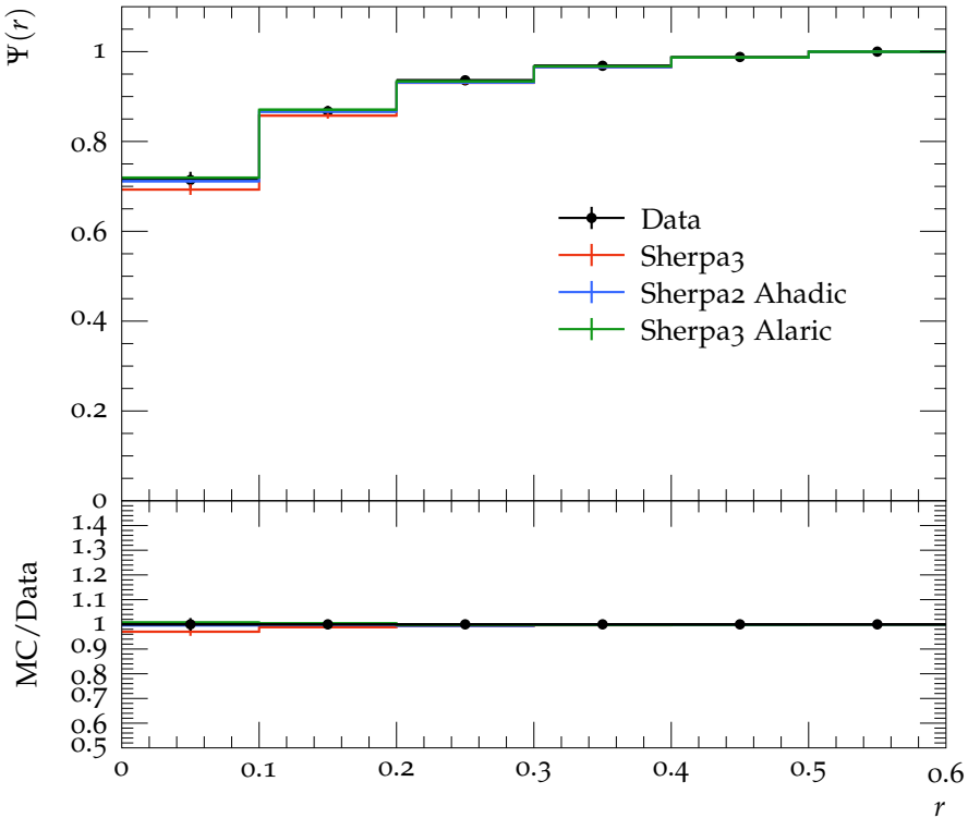
Jet shape \Psi for p_{\perp} \in 260\text{--}310\text{ GeV} , y \in 0.0\text{--}0.3
