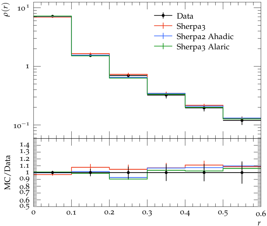
Jet shape \rho for p_{\perp} \in 260\text{--}310 GeV, y \in 0.0\text{--}0.3
