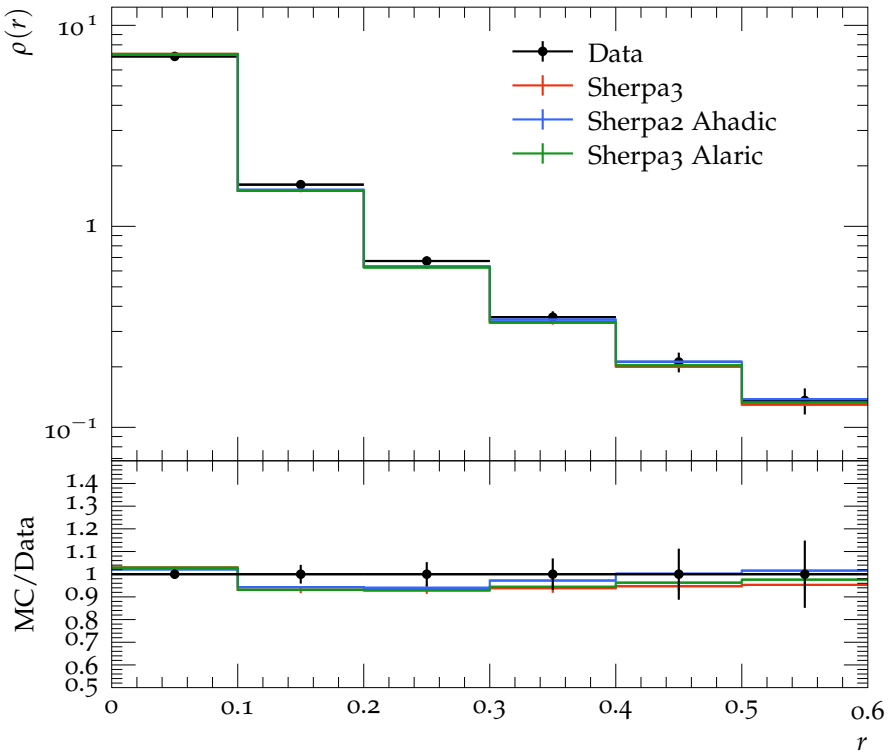
Jet shape \rho for p_{\perp} \in 210\text{--}260 GeV, y \in 0.0\text{--}2.8
