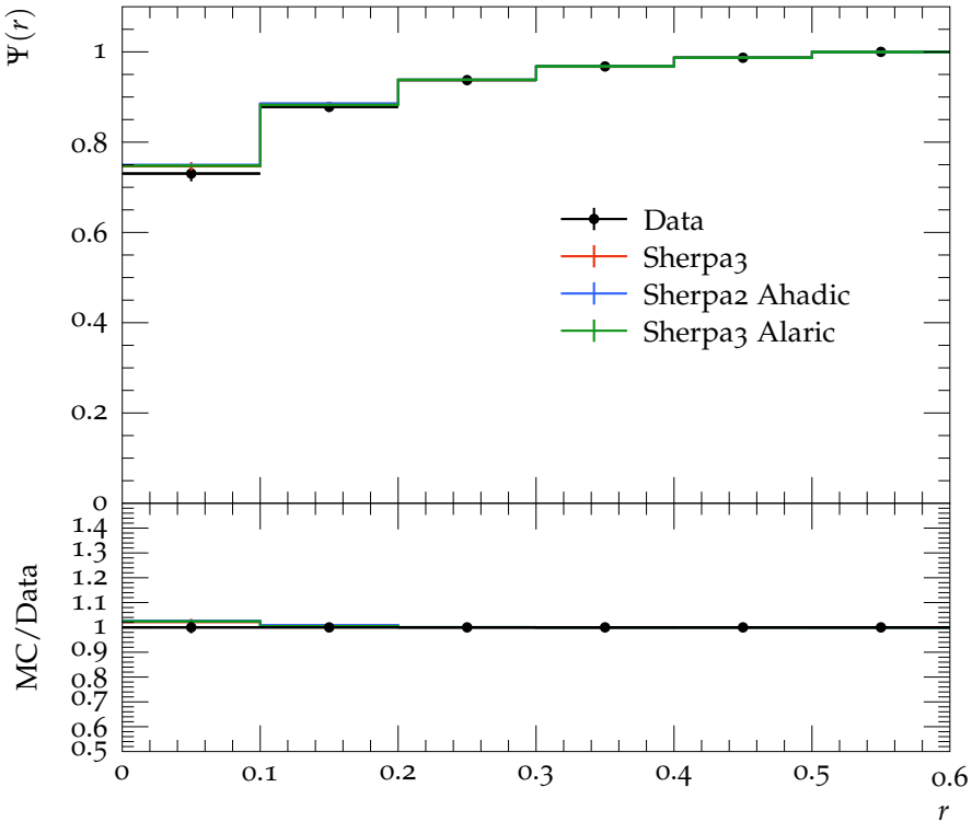
Jet shape \Psi for p_{\perp} \in 160\text{--}210\text{ GeV} , y \in 2.1\text{--}2.8
