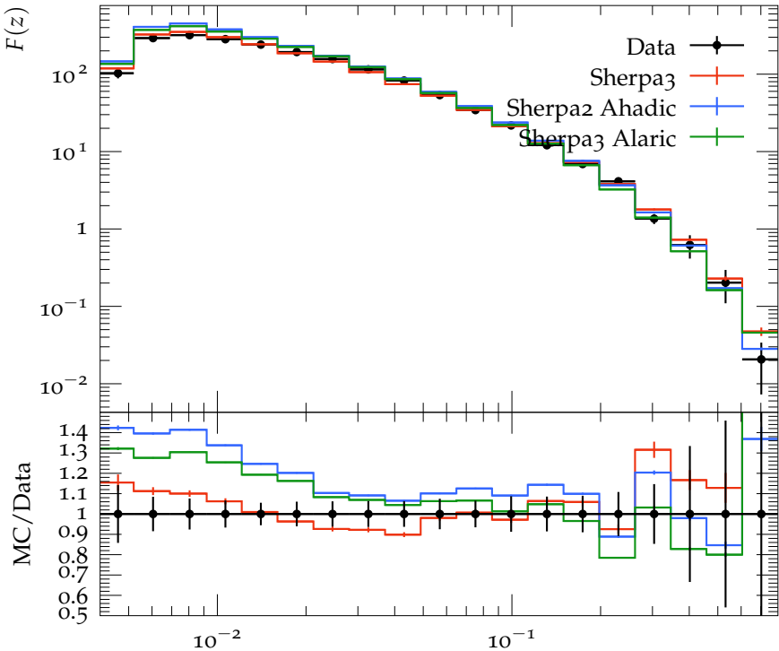
F(z) for 80 \text{ GeV} < p_{T \text{ jet}} < 110 \text{ GeV}
